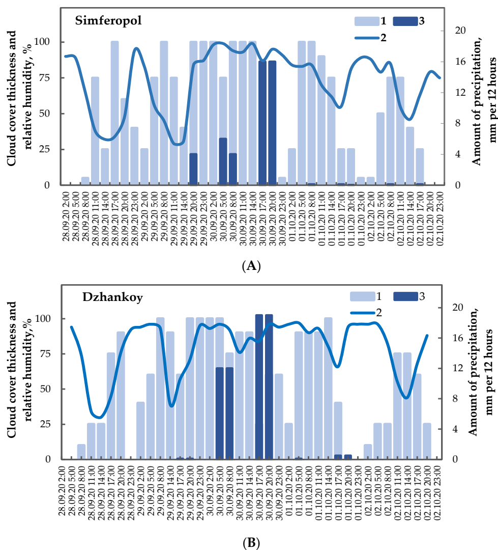
Figure 11. The daily variation in cloud cover thickness (1—scale on the left), relative air humidity (2—scale on the left) and the amount of precipitation (3—scale on the right) at the Simferopol (A) and Dzhankoy (B) meteorological stations for the period from September 28 to October 2, 2020, as a result the passage of the cold front through the Crimean Peninsula and the active influence on atmospheric processes.
